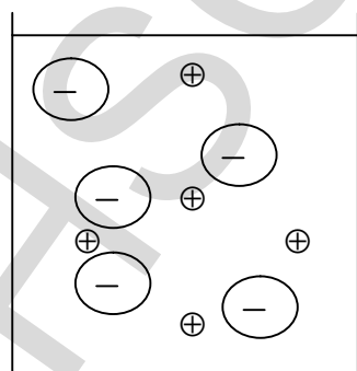
strong acid
